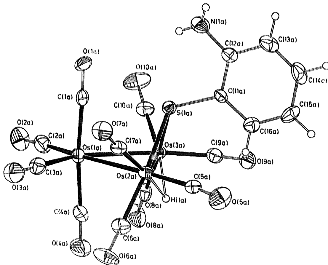
Fig. 1. A view of the molecular structure of one of the two crystallographically independent molecules found in one crystal of compound 3 . Thermal ellipsoids are drawn at the 30% probability level.
